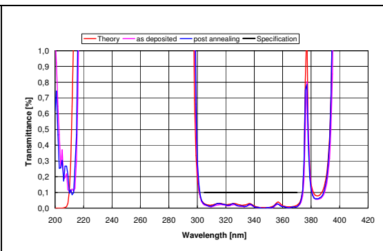
Figure 3b: Performance of the blocking band
